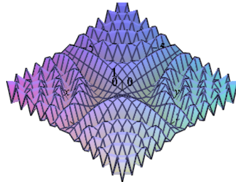
Abbildung 15: f(x, y) = \sin(xy)
