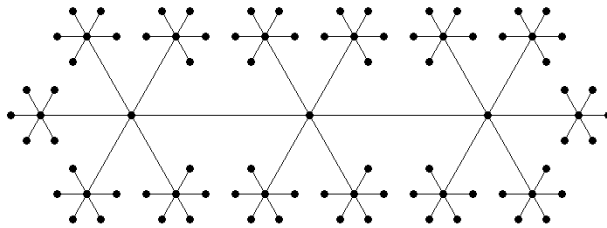
Figure 1: Part of the tree of local maximal orders for q = 5 .
