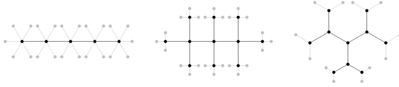
Figure 2: Subtree for \Phi_0(\pi^4) , in the cases q = 5, 3 and 2 .
