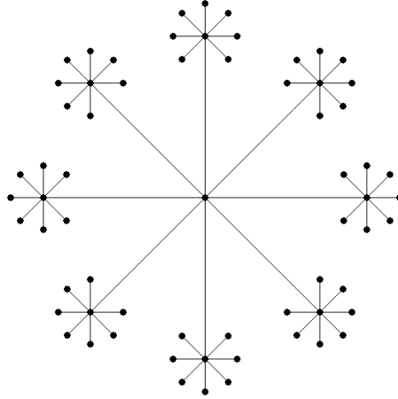
Figure 3: Subtree for \Phi(\pi^2) in the local algebra A_\pi for q = 7
