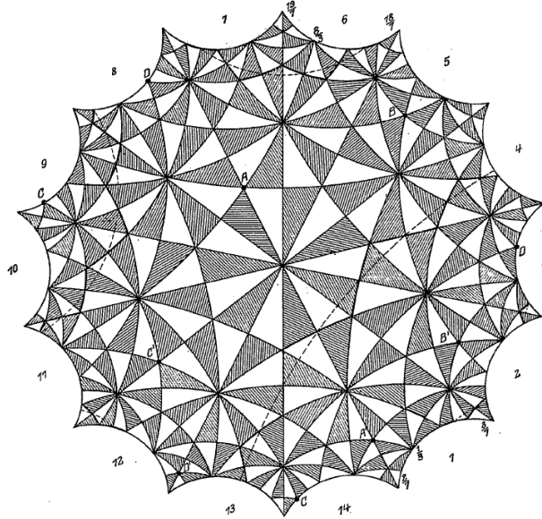
Figure 4: Klein's surface is obtained by the side pairing 1 \leftrightarrow 6 , 3 \leftrightarrow 8 , 5 \leftrightarrow 10 , 7 \leftrightarrow 12 , 9 \leftrightarrow 14 , 11 \leftrightarrow 2 , 13 \leftrightarrow 4 .
