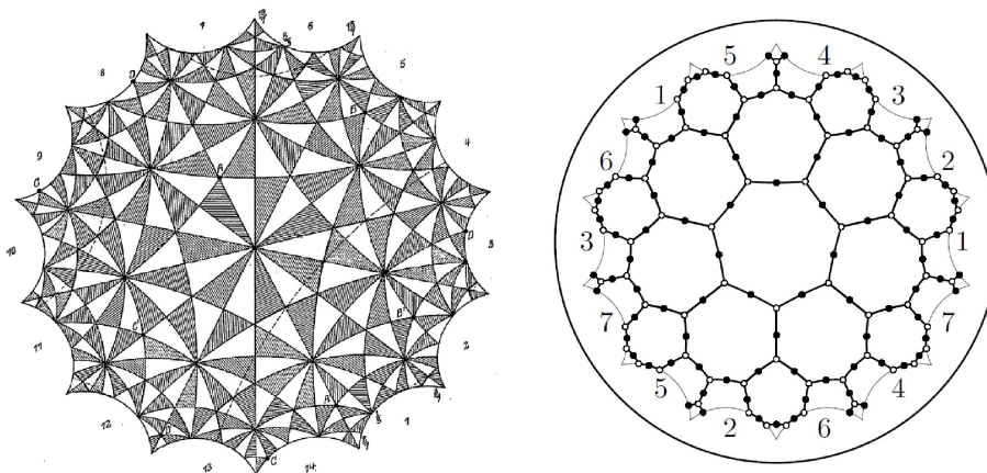
Figure 1: Tesselation and dessin for Klein's quartic x^3y + y^3z + z^3x = 0
