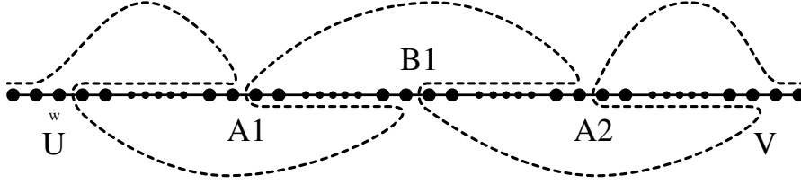
FIGURE 1. \mathcal{H}^* for r = 3 and \ell = 3 . The vertices of \mathcal{D}_\ell^{(r)} are drawn bigger than the vertices newly inserted in \mathcal{H} . The continuous line indicates the tight Hamilton path in \mathcal{H}^* from (13), the dashed line the tight Hamilton path in \mathcal{H}^* - w^* .
