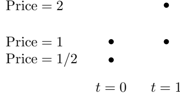
Figure 2: Deterministic model satisfying (NA^{wps}) but not (NA^{ps}) . One has \underline{S}_0 = 1/2 , \bar{S}_0 = 1 , \underline{S}_1 = 1 , and \bar{S}_1 = 2 .
